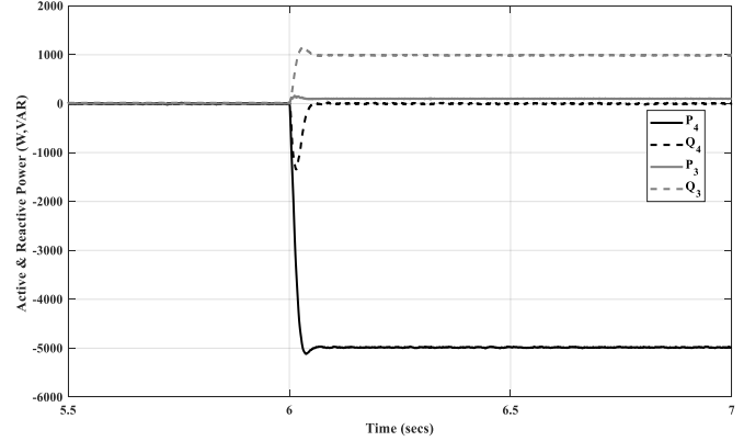
Fig. 12. Active and reactive power through the secondary and series winding during activation of the Secondary Current Controller.
