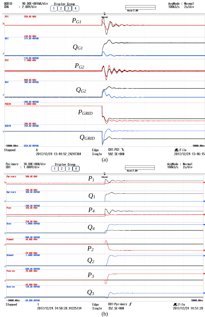
Fig. 22. Real-time simulation of the active and reactive power through the 5-bus power system with controllers disabled (black lines) and controllers enabled. (a) Grid sources and (b) CPAT windings (2sec/div).
