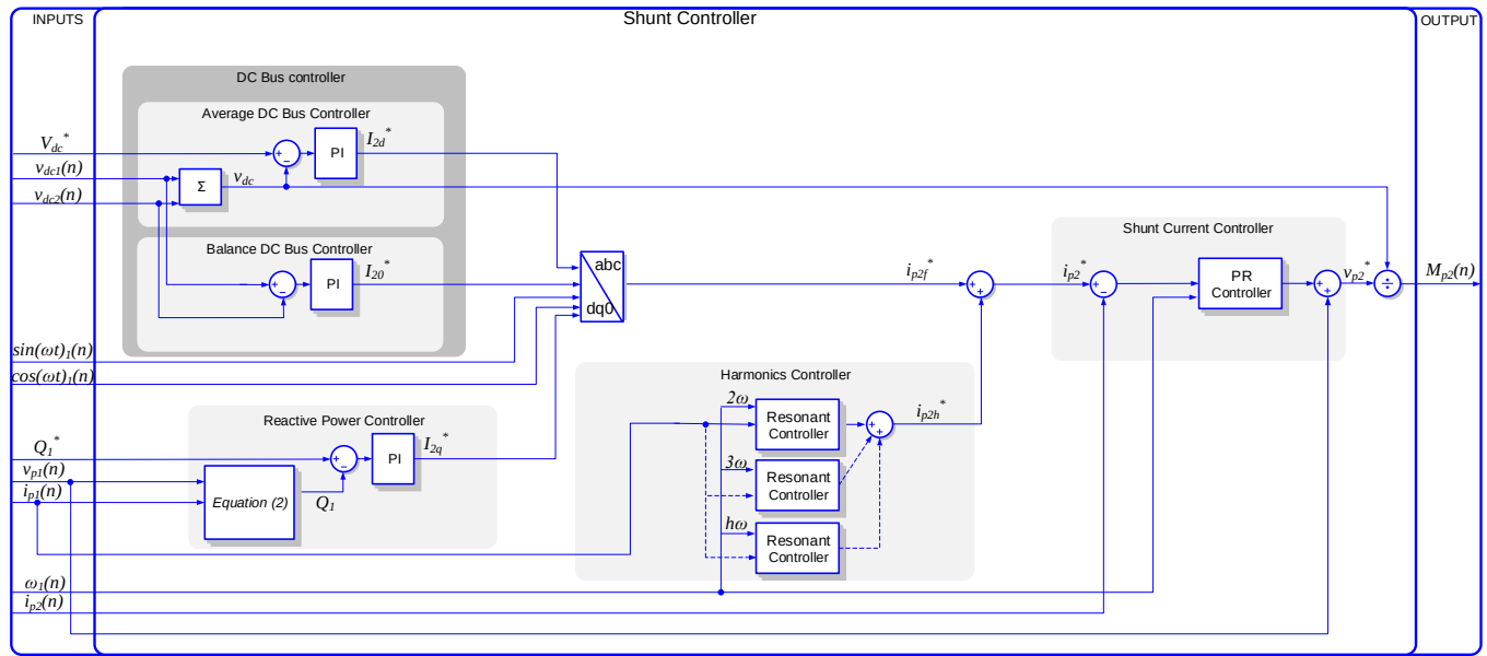
Fig. 6. Shunt Controller block structure.
